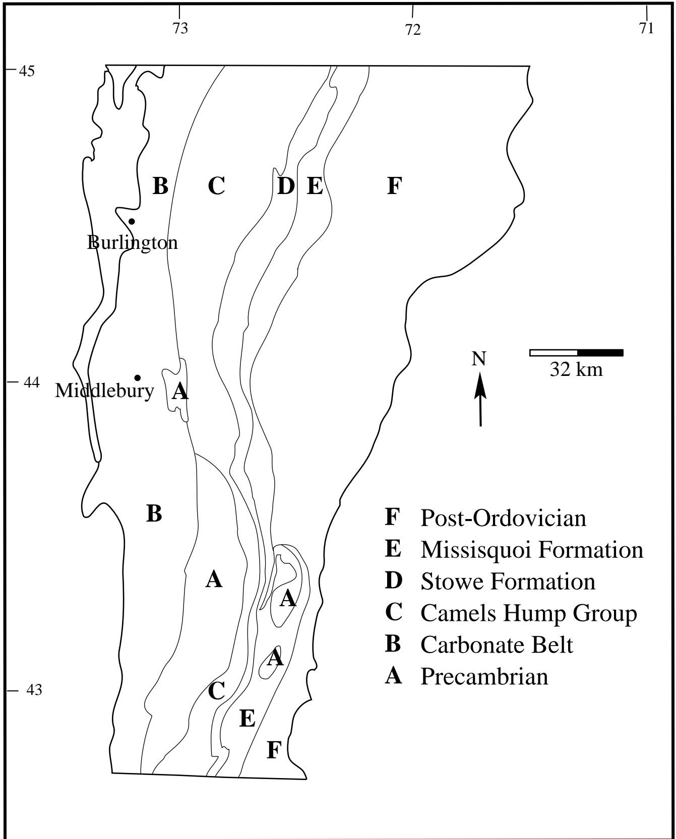
Fig. 1. Generalized geologic map of Vermont (after Doll et al., 1961)
