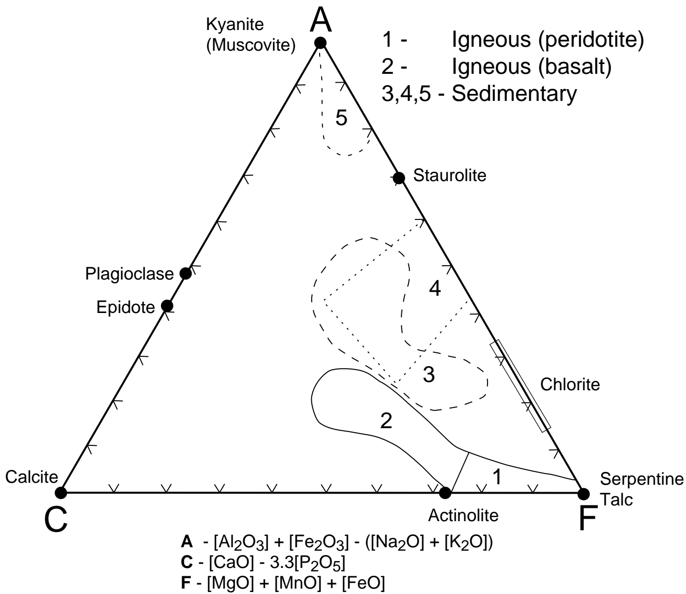
Protoliths for Metamorphic Rocks
